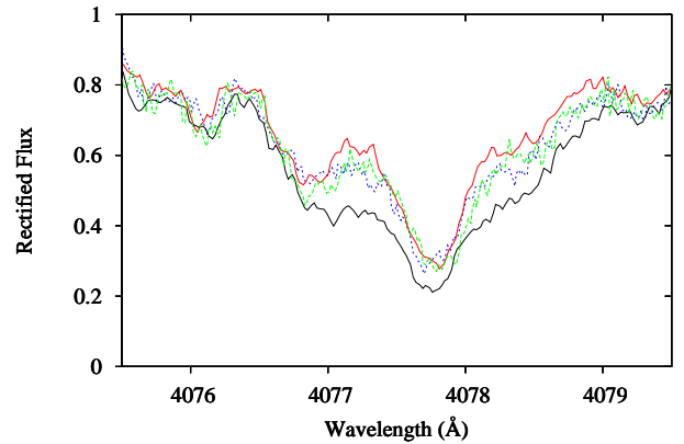
Figure 8. Variations in the profile shape of the Sr II 4077.7Å line with rotational modulation phase. The solid black line was taken at \phi_{\text{rot}} = 0.978 , the solid red line at \phi_{\text{rot}} = 0.597 . The dashed green and dotted blue lines were taken at \phi = 0.771 and \phi_{\text{rot}} = 0.227 , respectively.
