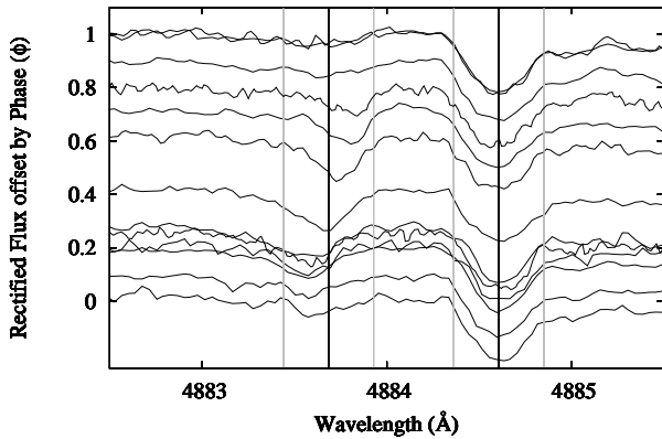
Figure 9. Changes in line profile strength and shape with rotational phase for the Y II line at 4883.7\text{\AA} . The rectified spectra have been offset so that their continuum levels correspond to their rotational phases. The nearby Cr II line at 4884.6\text{\AA} shows little shape variation with phase. The vertical black and grey lines indicate the line centres and the \pm 15 \text{ km s}^{-1} v \sin i widths, respectively.
