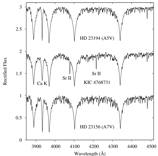
Figure 1. Spectrum of KIC 4768731 compared to the A5V and A7V MK standards. Note the prominent Sr II lines at 4077\text{\AA} and 4216\text{\AA} and the abnormal Ca II K line. The spectra have been offset for clarity.
