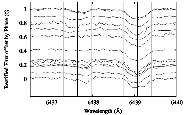
Figure 10. Changes in line profile strength and shape with rotational phase for the Eu II line at 6437.6\text{\AA} . The rectified spectra have been offset so that their continuum levels correspond to their rotational phases. The nearby Ca I line at 6439.1\text{\AA} shows little shape variation with phase. The vertical black and grey lines indicate the line centres and the \pm 15 \text{ km s}^{-1} v \sin i widths, respectively.
