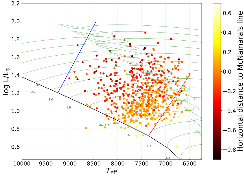
Figure 5. HR diagram for our sample of Kepler \delta Sct stars having fractional parallax uncertainties less than 5 percent and pulsation semi-amplitudes above 1 mmag. Luminosities and temperatures are taken from Murphy et al. (2019). The colour indicates the horizontal distance from the fundamental-mode relation in the P–L diagram (Fig. 4), with redder colours corresponding to shorter periods (higher pulsation overtones). The evolutionary tracks (green) are from Murphy et al. (2019) and have X = 0.71 and Z = 0.014 . The blue and red lines are the theoretical instability strip boundaries using TDC and \alpha_{\text{MLT}} = 1.8 from Dupret et al. (2005).
