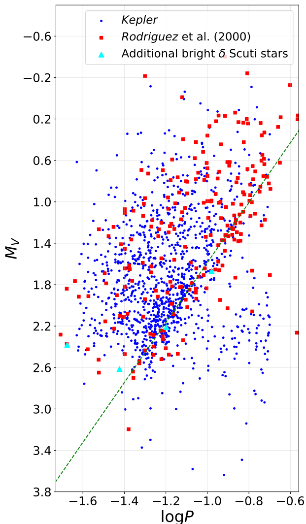
Figure 1. Period–luminosity diagram of \delta Sct stars having fractional parallax uncertainties less than 5 percent. Blue dots are 1124 \delta Sct stars in the Kepler field and red squares are 228 stars from the \delta Sct catalogue of Rodríguez et al. (2000). The cyan triangles indicate the four additional bright \delta Sct stars discussed in Sec. 2.1, which are (from left to right) \beta Pic, \eta Ind, Altair and 95 Vir. The diagonal dashed green line shows the relation from McNamara (2011, see Eq. 3).
