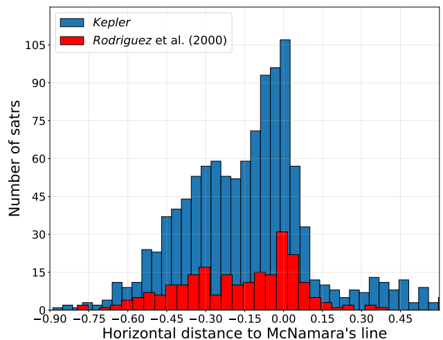
Figure 2. The distance of data points to the McNamara line as a histogram. Red: 228 \delta Sct stars from Rodríguez et al. catalogue corrected for extinction by Green et al. (2015) dust map. Blue: 1124 \delta Sct stars from Kepler , corrected for extinction by the Green et al. (2018) dust map.
